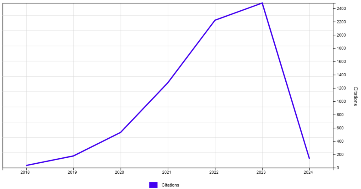
Figure 5 Citations
