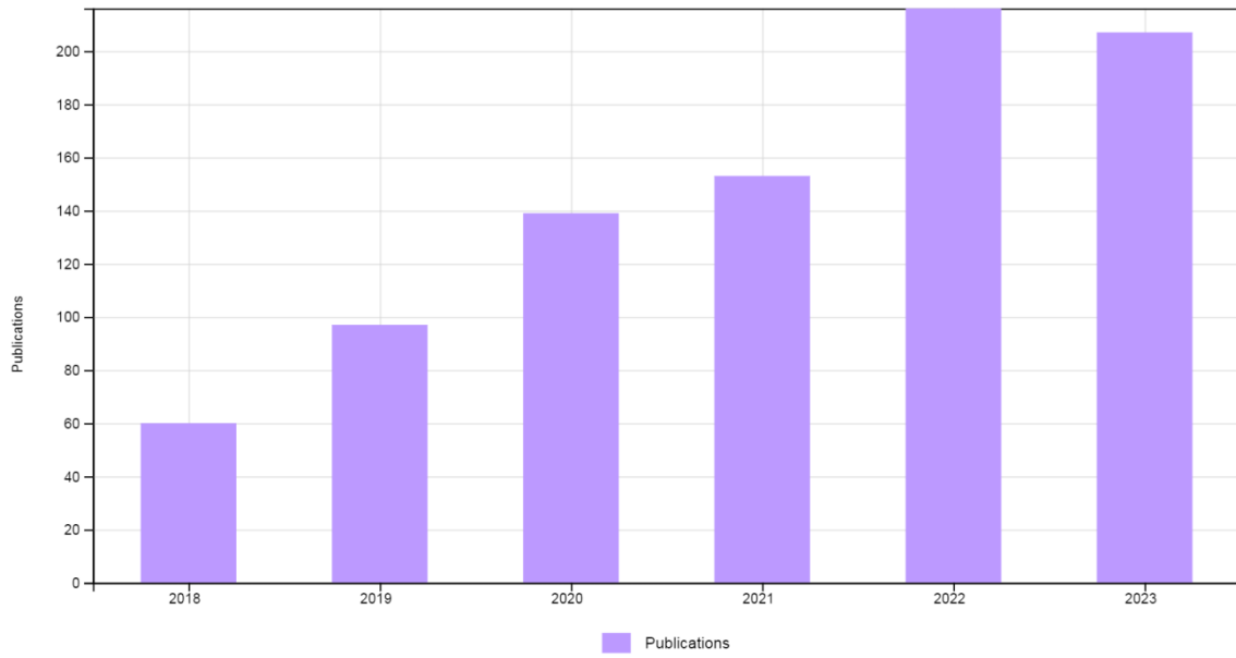
Figure 4 Publications
